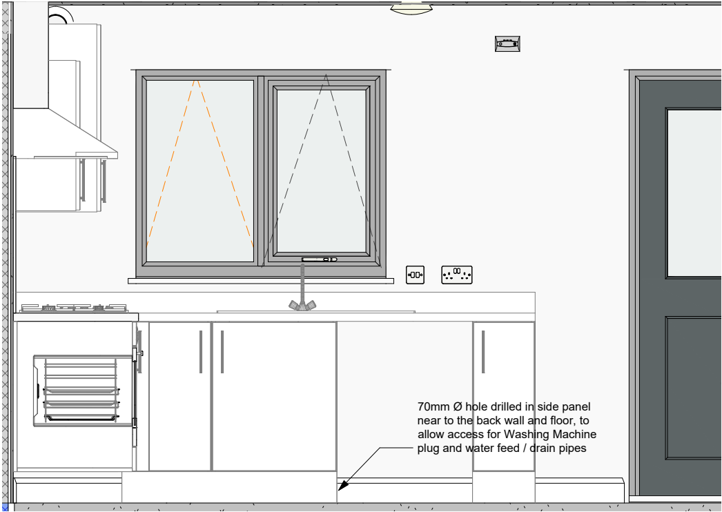
C Kitchen - View C (Shared Ownership Spec) 1 : 25
