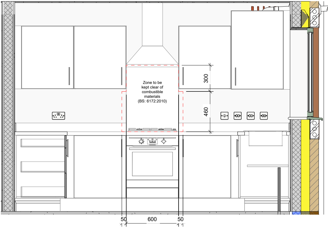
B Kitchen - View B (Shared Ownership Spec) 1 : 25
